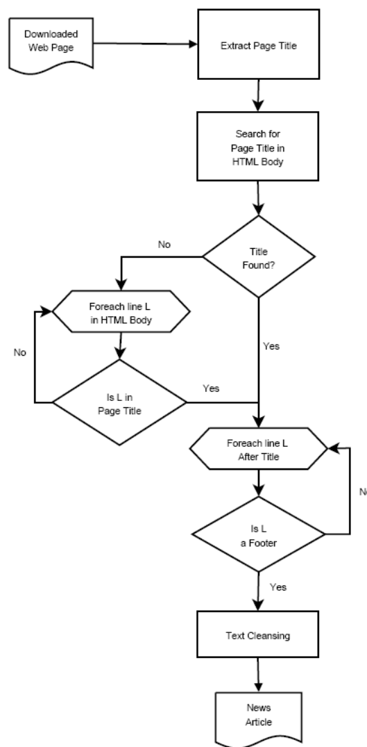
Fig. 3 overview of rule based extraction
