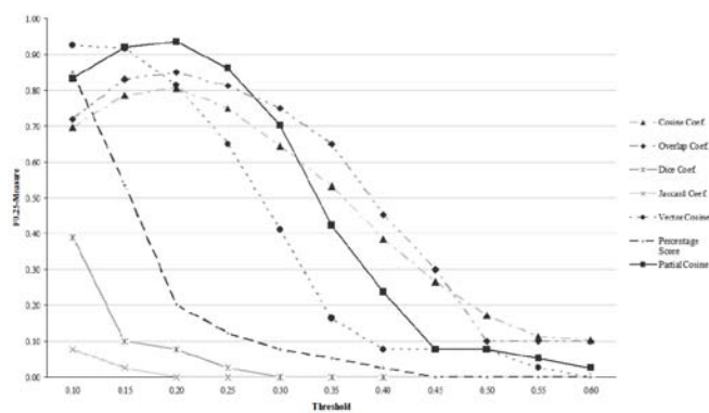
Fig. 5 similarity results for English
