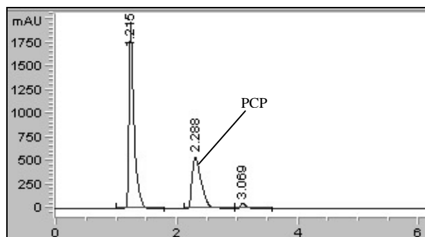
Fig. 4 HPLC chromatogram for SBR influent
