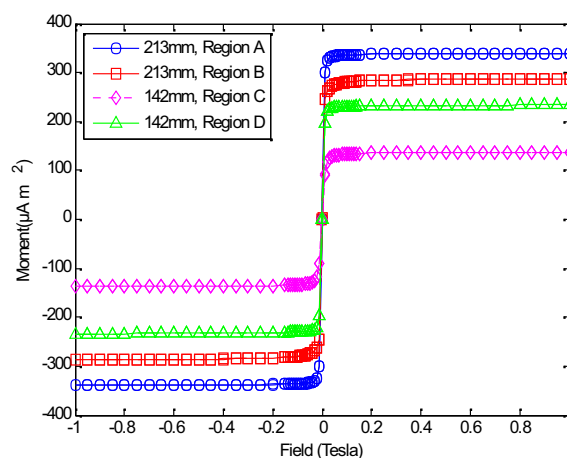
Fig. 7 The measured results of magnetic properties identified by VSM
