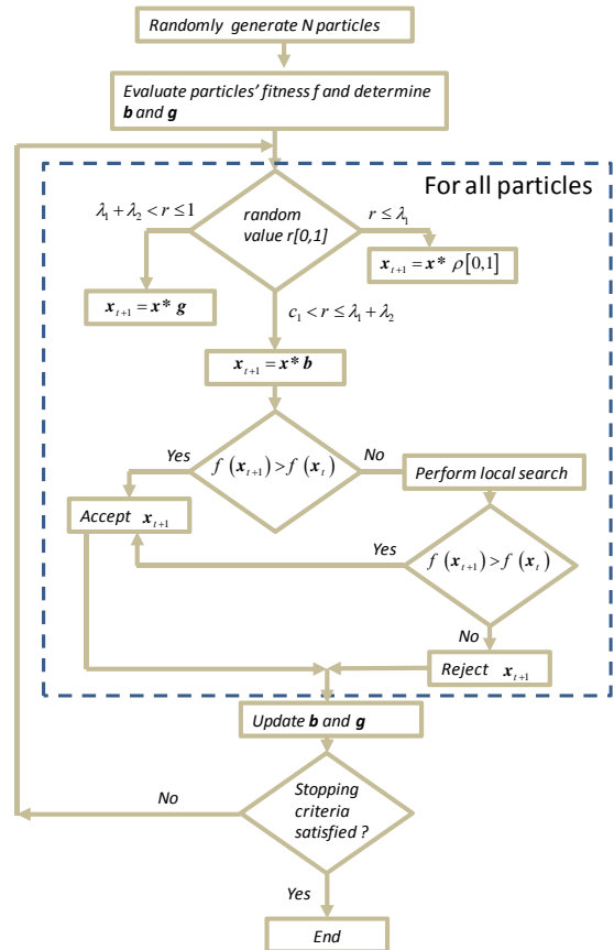
Fig. 2 Flowchart describing JPSO algorithm
