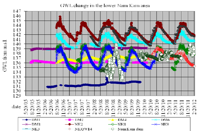
Fig. 3 Groundwater level change from 2005 to 2012
