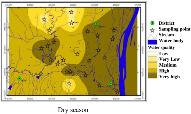
Fig. 12 Surface water quality assessment evaluate using SAR
