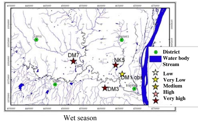
Fig. 13 Shallow groundwater water quality assessment evaluate using SAR
