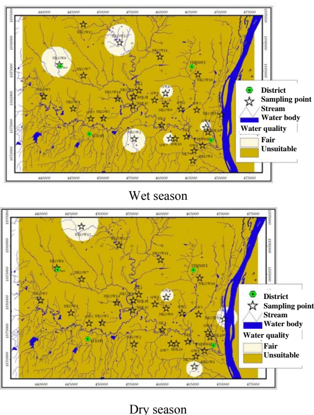
Fig. 18 The assessment of suitability of shallow groundwater
