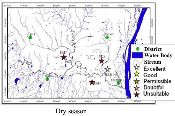
Fig. 11 Deep Groundwater quality assessment evaluate using EC_w
