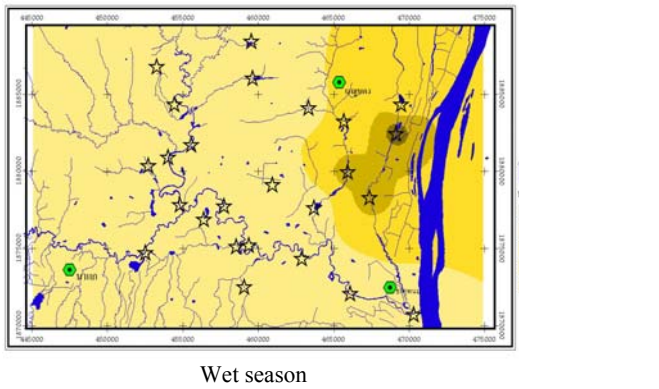
Fig. 11 Deep Groundwater quality assessment evaluate using EC_w
