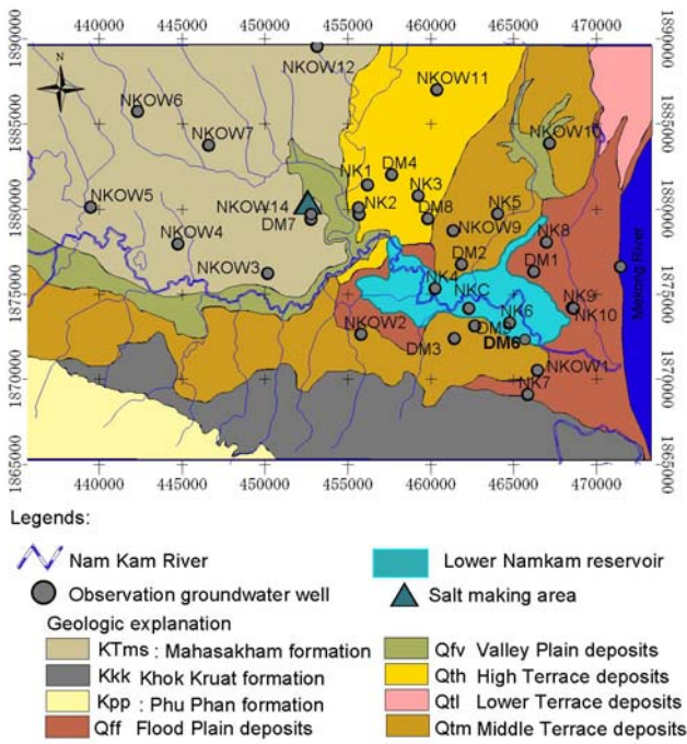
Fig. 2 Geologic map of Lower Nam Kam River Basin
