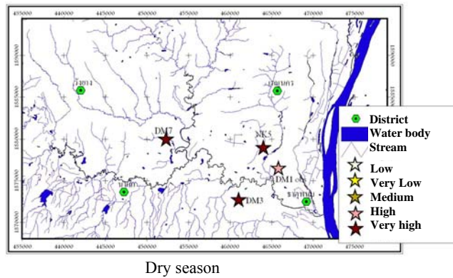
Fig. 14 Deep groundwater water quality assessment evaluate using SAR
