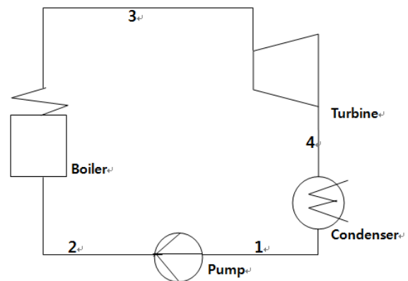
Fig. 1 Rankine Cycle
