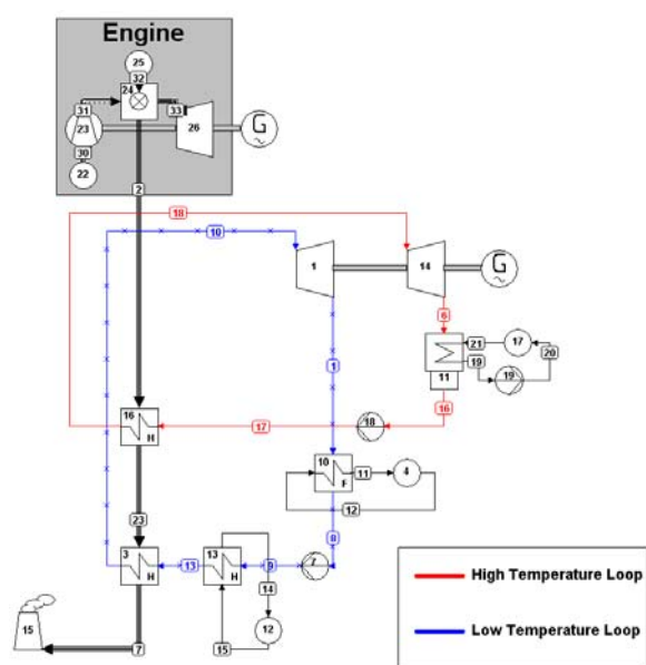
Fig.11 schematic of co-generation system used for simulation
