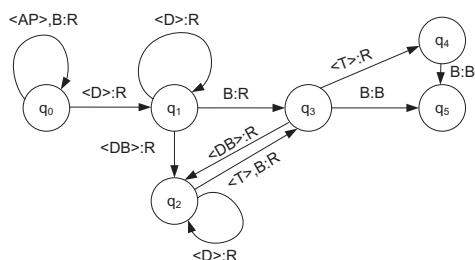
Fig. 10. Turing machine for courtesy amount interpretation.
