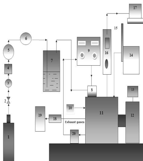
Fig. 3 Schematic layout of the experimental setup
