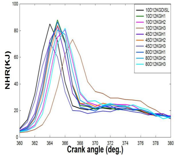
Fig. 6 Neat heat release (NHR) vs crank angle at full load
