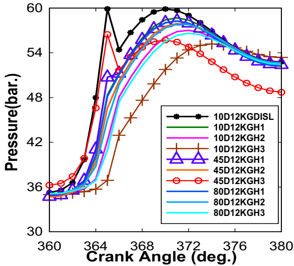
Fig. 4 Pressure vs crank angle at full load
