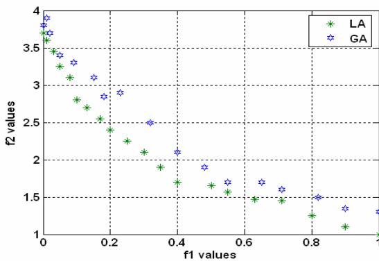
Fig. 2 The results of optimization of \vec{F}_1 by LA-based and GA-based methods
