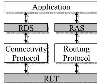
Fig 1: MASGRID Architecture
