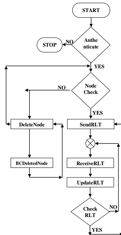
Fig 5: Resource Discovery Algorithm
