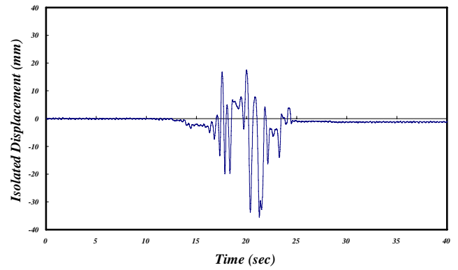
Fig. 26 Time history of isolator displacement under Chi-Chi earthquake with 0.540g in PGA
