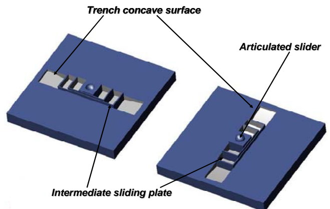
Fig. 3 Open-up view of MTFPS Isolator
