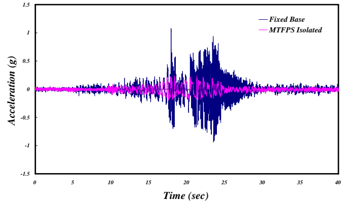
Fig. 20 Comparison of roof acceleration responses of fixed- base and MTFPS-isolated structures under Chi-Chi earthquake with 0.540g in PGA
