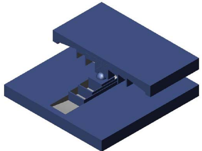
Fig. 2 Exploded view of MTFPS Isolator
