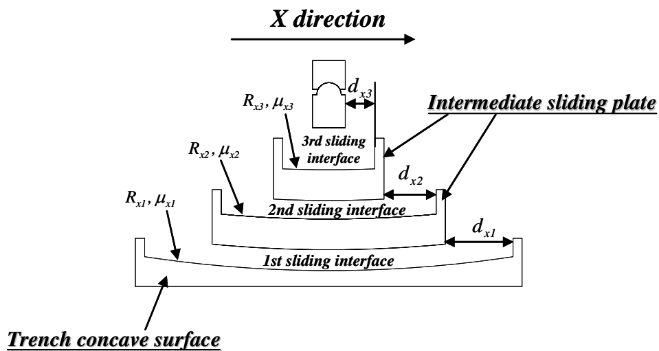
Fig. 6 Properties of sliding interfaces in MTFPS isolator
