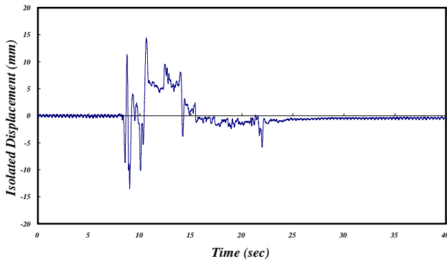
Fig. 24 Time history of isolator displacement under El Centro earthquake with 0.619g in PGA
