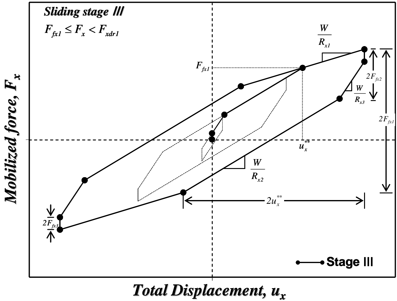
Fig. 12 Force-displacement relationship of the MTFPS isolator during Stage III
