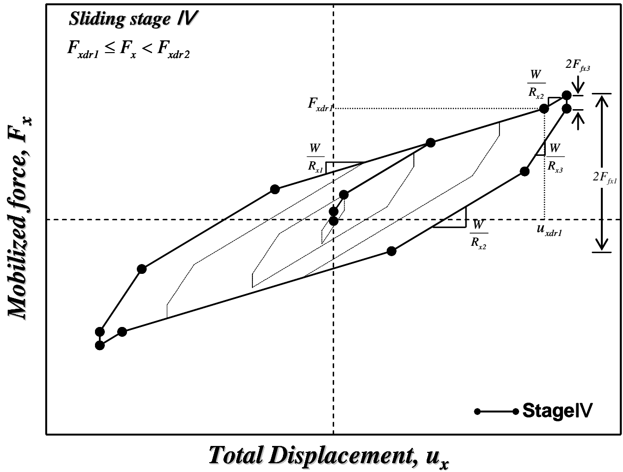
Fig. 14 Force-displacement relationship of the MTFPS isolator during Stage IV
