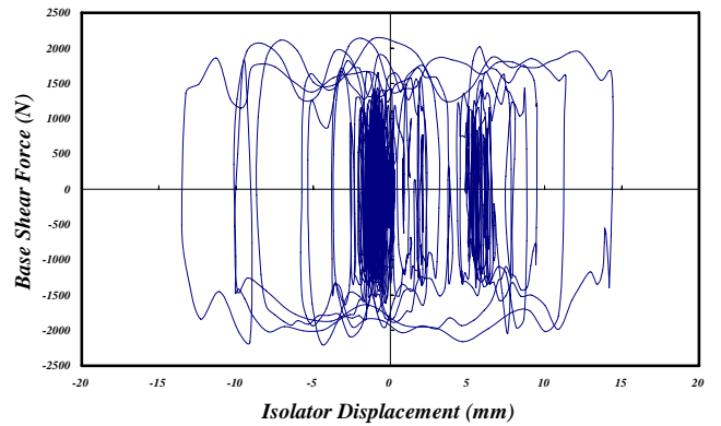
Fig. 21 Hysteresis loops of base isolator under El Centro earthquake with 0.619g in PGA
