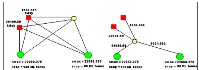
Fig. 4 Solution of the CO 2 transport grid for the Lazio Area
