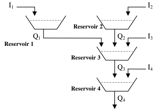
Fig. 1 Hydraulic network for studies
