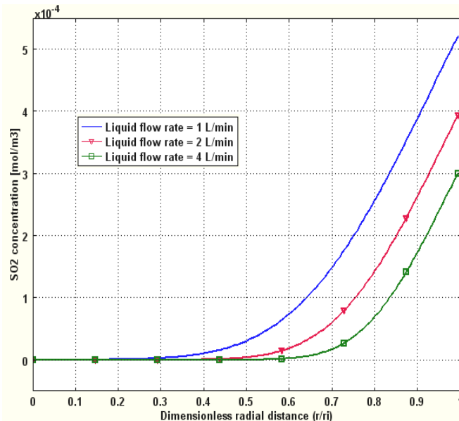
Fig. 4 Effect of liquid flow rate on SO 2 concentration profile in the tube side
