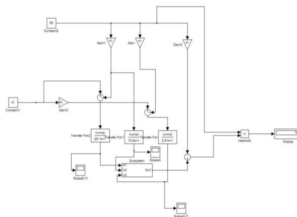
Fig. 2 SOFC model for pressure test
