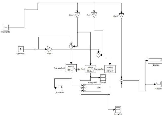
Fig. 3 SOFC model for power test
