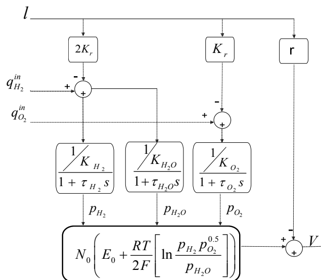
Fig. 1 SOFC stack dynamic model
