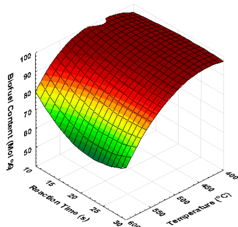
Fig. 6 The change of total biofuel content with temperature and reaction time, for Pt/Al 2 O 3 catalyst
