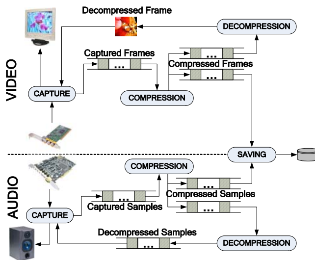
Fig. 2 Computacional elements of the prototype
