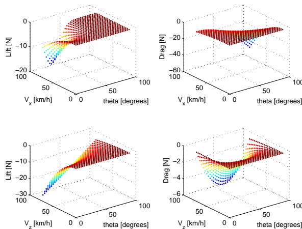
Fig. 10. The Lift and Drag Forces Created by the Wings
