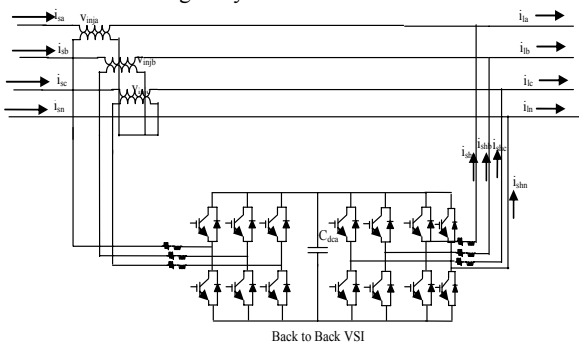
Fig. 2 UPQC Block Diagram
