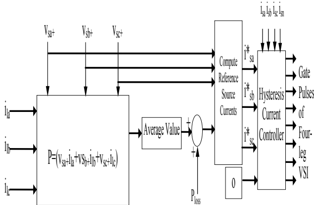
Fig. 4 Control Scheme of Shunt APF using ISCT
