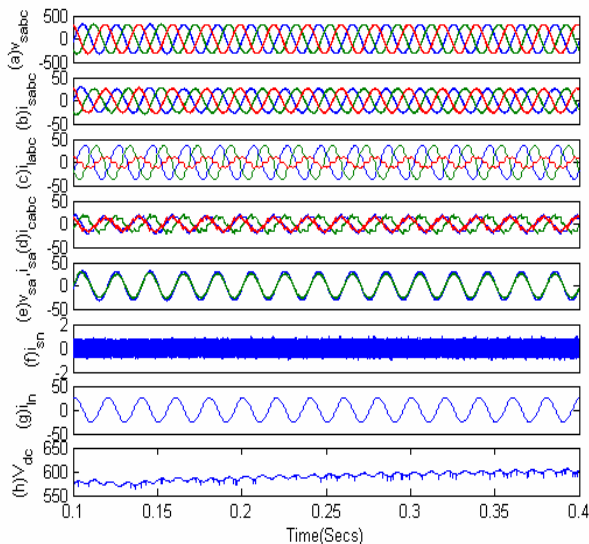
Fig. 6 Performance of UPQC for load balancing, power factor correction and current harmonic mitigation
