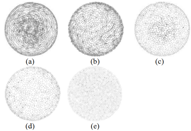
Fig. 3 (a) v_p at pipe inlet section, (b) v_p at pipe exit section at t_p=1 mm, (c) v_p at pipe exit section at t_p=3 mm, (d) v_p at pipe exit section at t_p=6 mm and (e) v_p at pipe exit section at t_p=12 mm
