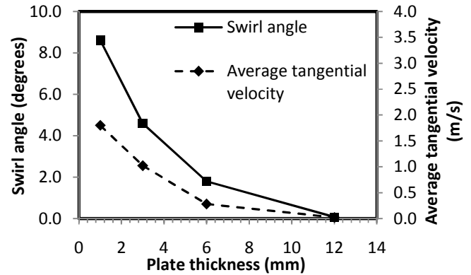
Fig. 4 Average tangential velocity and swirl angle at pipe outlet for different plate thicknesses
