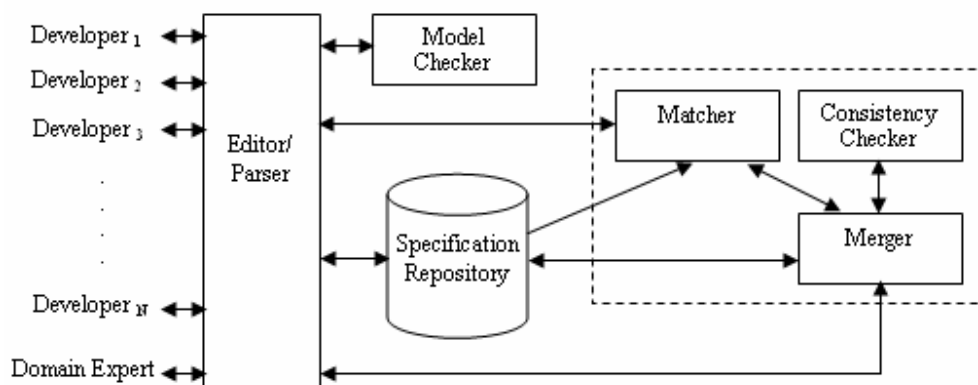
Fig. 1 Architecture of the proposed framework
