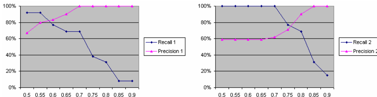
Fig. 5 Matching results for the two views of the online purchase system
