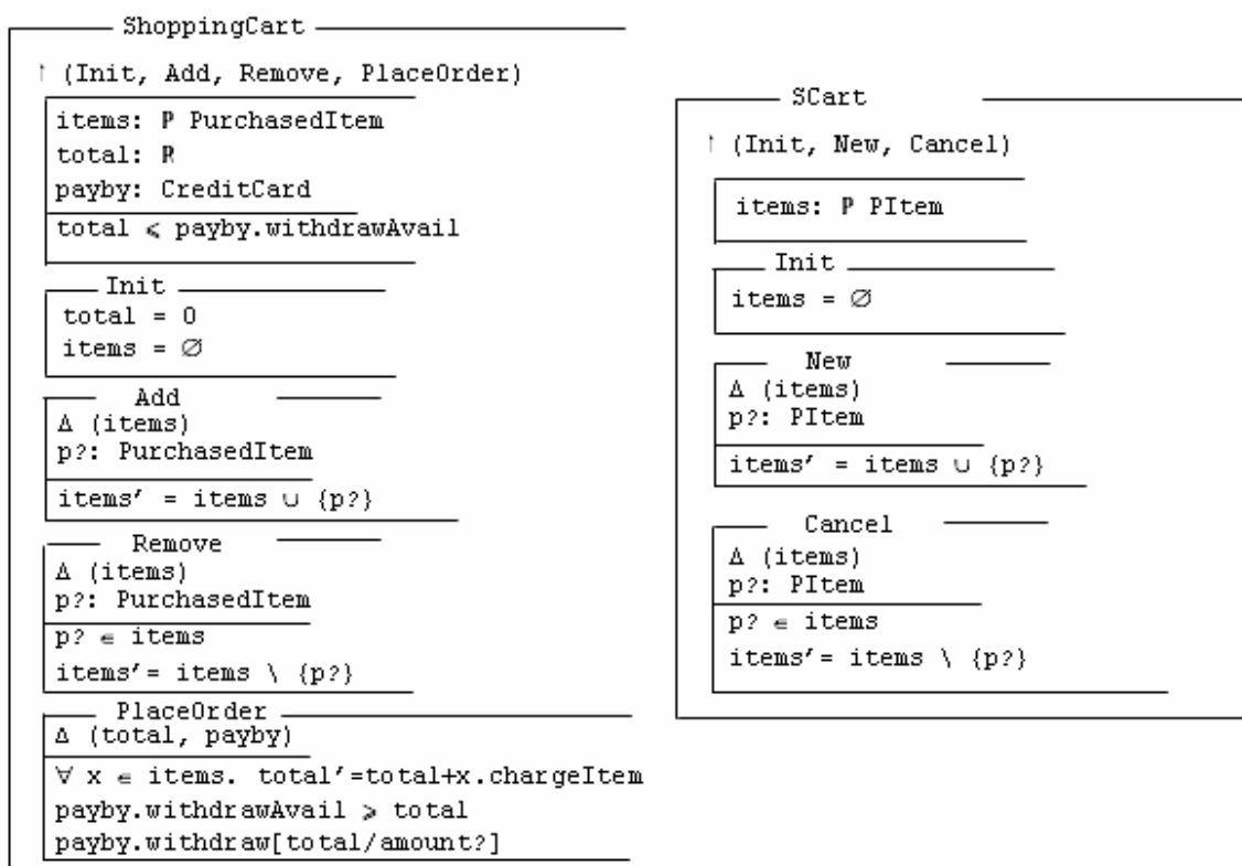
Fig. 2 Two views of an Object-Z class
