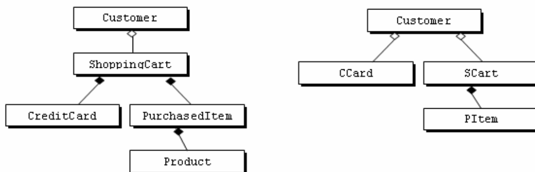
Fig. 3 The classes and their relationships of two views of the same system
