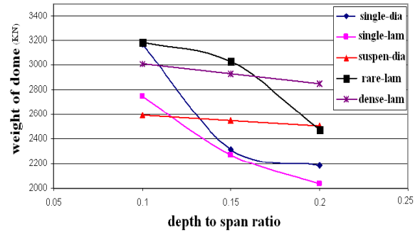
Fig. 11 Comparison of models weight
