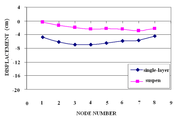
Fig. 6 Deflection of objective nodes in diamatic domes under symmetric snow load
