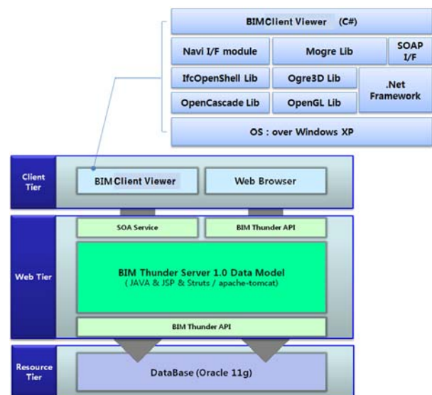
Fig. 4 Architecture of the BIM Server and Viewer
