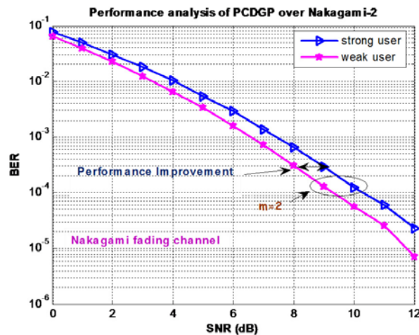
Fig. 3. Simulation results for the PCDGP system for both users over Nakagami-2 fading channel
