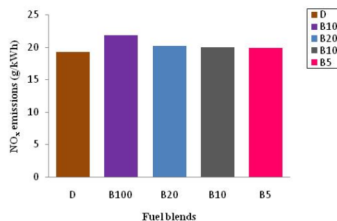
Fig. 3 Comparison of \text{NO}_x emissions for diesel and biodiesel-diesel blends at full load
