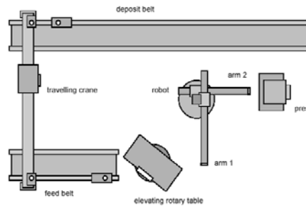
Fig. 3. Production Cell
