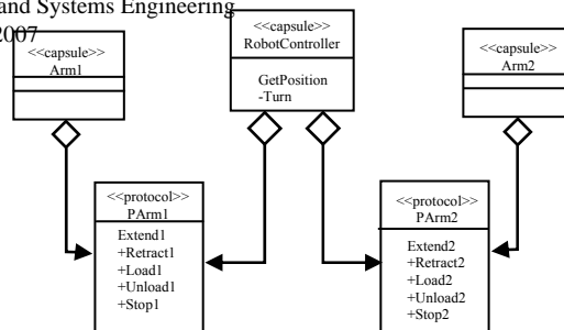
Fig. 5 The Robot component class
