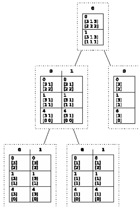
Fig. 6 Query Tree Evaluation
