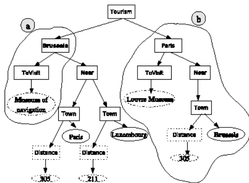
Fig. 7 Keyword Proximity
