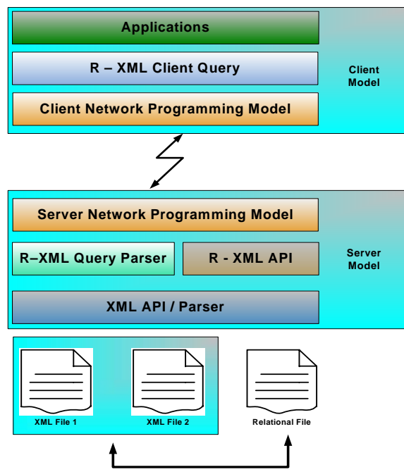
Fig. 9 R-XML Architecture
