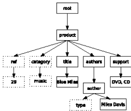
(a) XML-graph associated with the document doc_0
