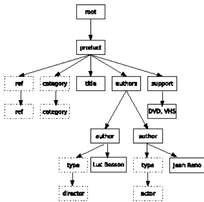
(b) XML-graph associated with the document doc_1
