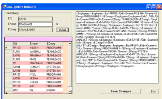
Fig. 8 Implementation of an indexing and querying method over XML document
