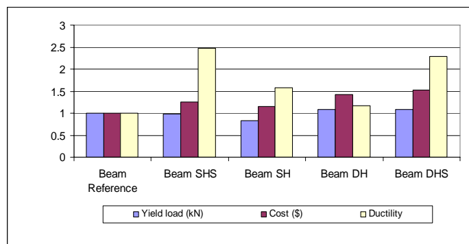
Fig. 7 Beam cost VS Ductility and strength
