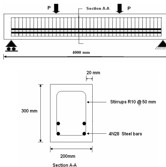
Fig. 2 Reference beam details
