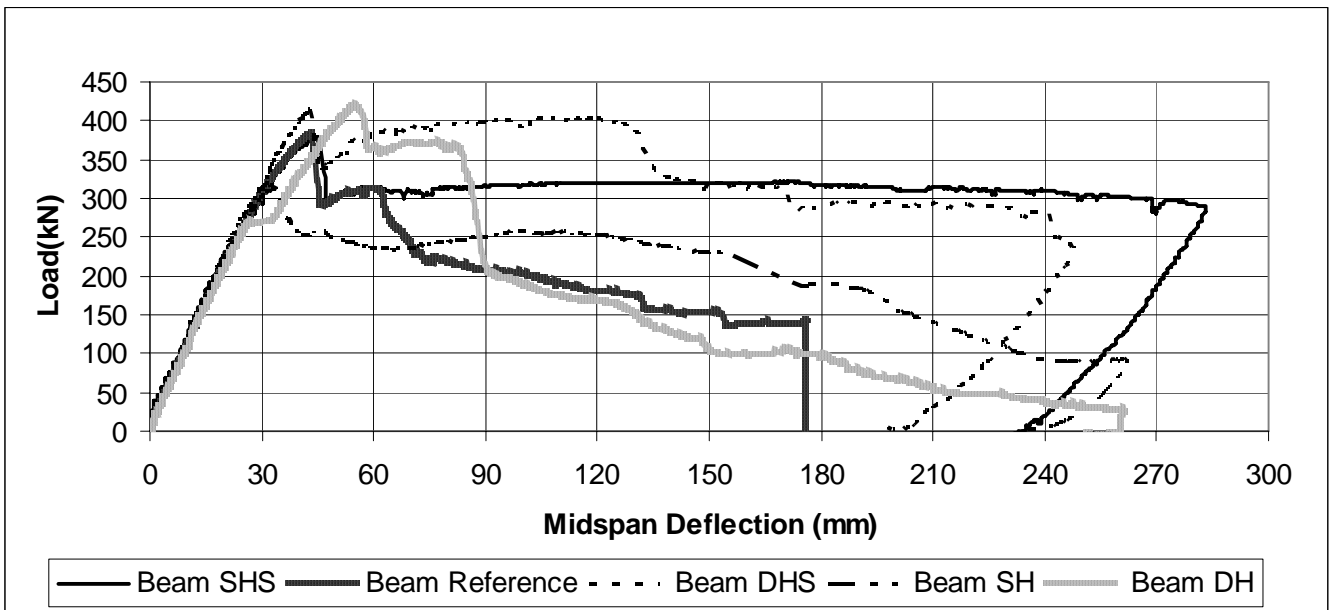
Fig. 5 Load vs Deflection at midspan for all five beams
