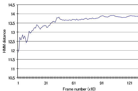
Fig. 9. HMM distance measure between /a/ and /e/ vowels.
