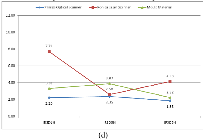
Fig. 5 Graph of percentage error of volume computed using midpoint projection algorithm
