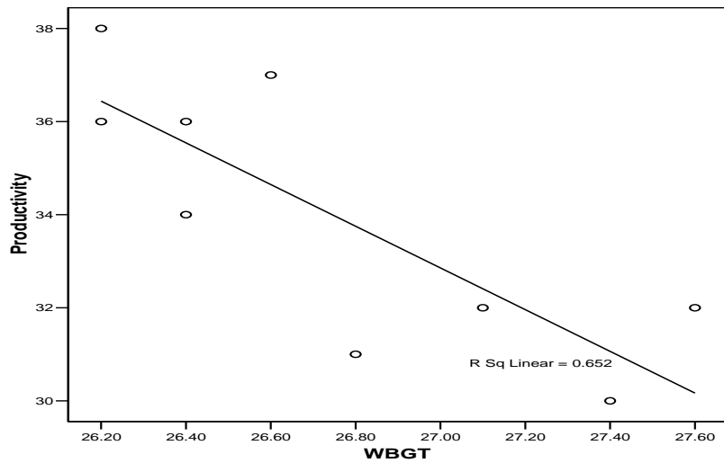
Fig. 5 Graph of Production Rate versus WBGT
