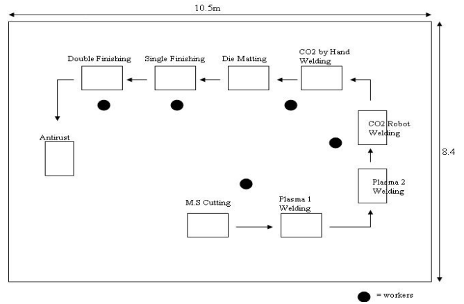
Fig. 3 Workstation Layout
