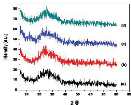
Fig. 5: X-ray diffraction patterns of VOPc thin films thermally deposited on glass substrates: (a) pristine and annealed at (b) 95°C, (c) 125°C and (d) 155°C.
