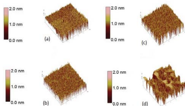
Fig. 3: 3-D AFM topographic images of VOPc thin films thermally deposited on glass substrates; scan size is 5\ \mu\text{m} \times 5\ \mu\text{m} : (a) pristine and annealed at (b) 95^\circ\text{C} , (c) 125^\circ\text{C} and (d) 155^\circ\text{C} .
