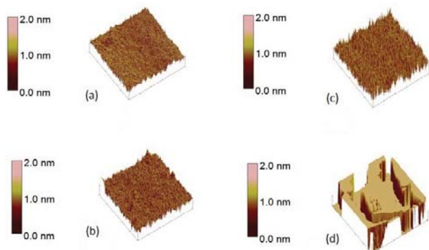
Fig. 2: 3-D AFM topographic images of VOPc thin films spin coated on glass substrates; scan size is 5\ \mu\text{m} \times 5\ \mu\text{m} : (a) pristine and annealed at (b) 95^\circ\text{C} , (c) 125^\circ\text{C} and (d) 155^\circ\text{C} .
