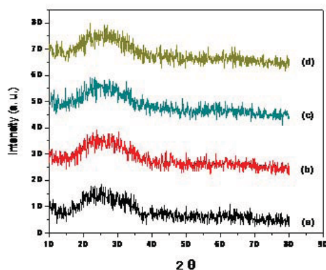
Fig. 4: X-ray diffraction patterns of VOPc thin films spin coated on glass substrates: (a) pristine and annealed at (b) 95°C, (c) 125°C and (d) 155°C.
