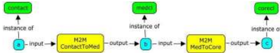
Fig. 8. Code generation through M2M mapping
