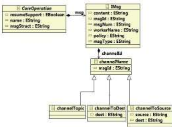
Fig. 6. The msgc1 meta-model
