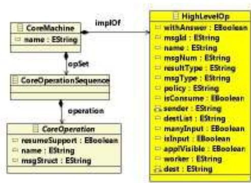
Fig. 9. corecl extension
