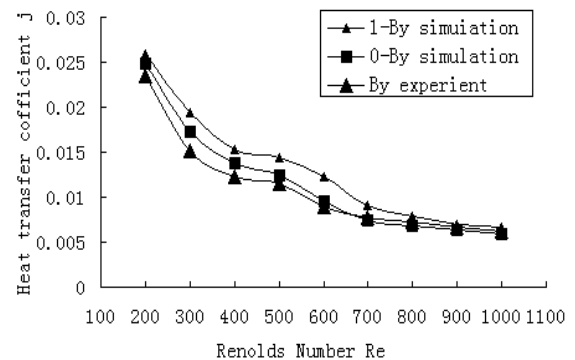
Fig. 9 Comparison of f in numerical simulation with experimental results 1- with corrugations; 0- without corrugations
