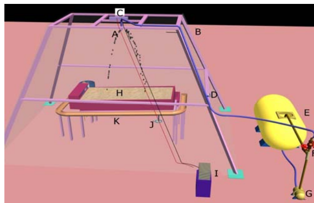
Fig. 1 Rainfall simulator (back view)
