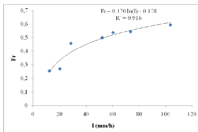
Fig. 5 Froude number versus rainfall intensity
