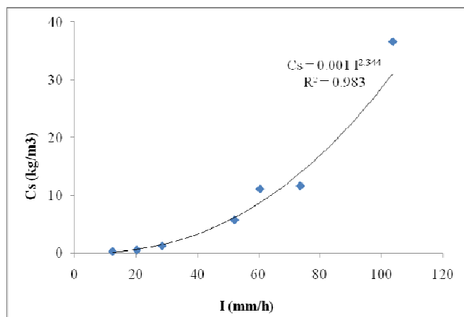
Fig. 7 Sediment concentration versus rainfall intensity
