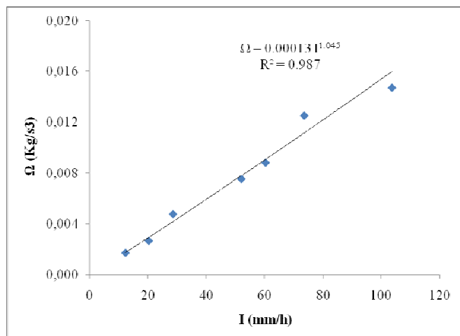
Fig. 6 Power flow versus rainfall intensity
