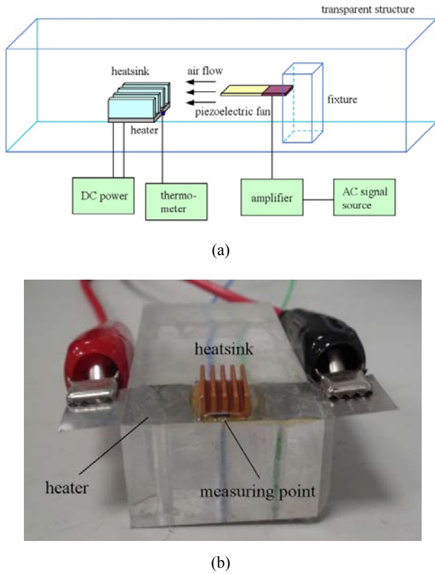
Fig. 13 Experimental equipments for cooling performance (a) layout figure (b) photo of heater and heatsink
