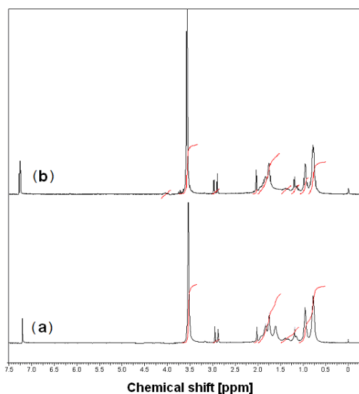
Fig. 2 1 H-NMR spectra of PMMA grafted cellulose in DMAc/LiCl solvent system in presence of BPO (Cell-g-PMMA-15) (a), PMMA grafted cellulose in DMAc/LiCl solvent system in presence of CAN (Cell-g-PMMA-70) (b)
