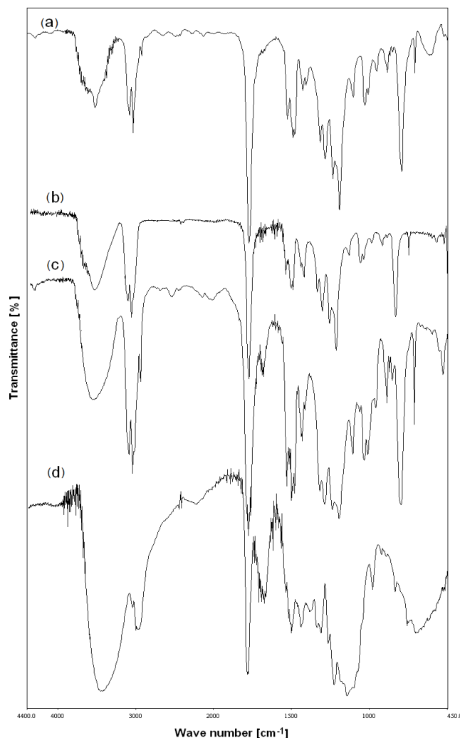
Fig. 1 FTIR spectra of PMMA grafted cellulose in DMAc/LiCl solvent system in presence of BPO (Cell-g-PMMA-15) (a), PMMA grafted cellulose in DMAc/LiCl solvent system in presence of Sn(Oct) 2 (Cell-g-PMMA-25) (b), PMMA grafted cellulose in DMAc/LiCl solvent system in presence of CAN (Cell-g-PMMA-70) (c), PMMA grafted cellulose in DMSO/PF solvent system in presence of CAN (Cell-g-PMMA-74) (d)
