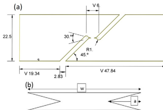
Fig. 4 (a) Loading frame (b) Effective test specimen
