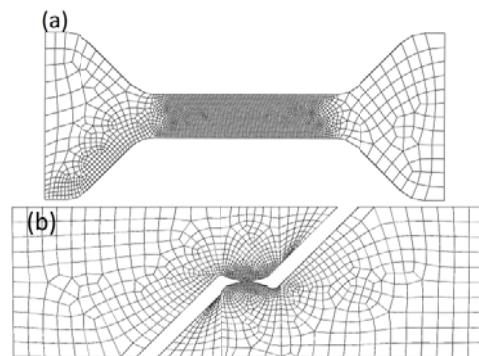
Fig. 8 Mash of tensile and shear specimen
