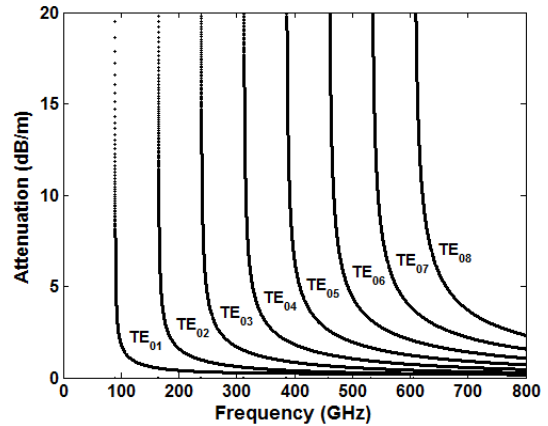
Fig. 3 Attenuation characteristics for different azimuthally symmetric modes TE_{0n} in a gyrotron cavity having electrical conductivity 5.8 \times 10^7 S/m
