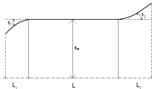
Fig. 1 Gyrotron cavity resonator
