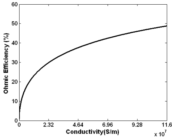
Fig. 5 Ohmic efficiency variations as a function of electrical conductivity of a 460 GHz gyrotron cavity wall excited in azimuthally symmetric mode TE_{06}
