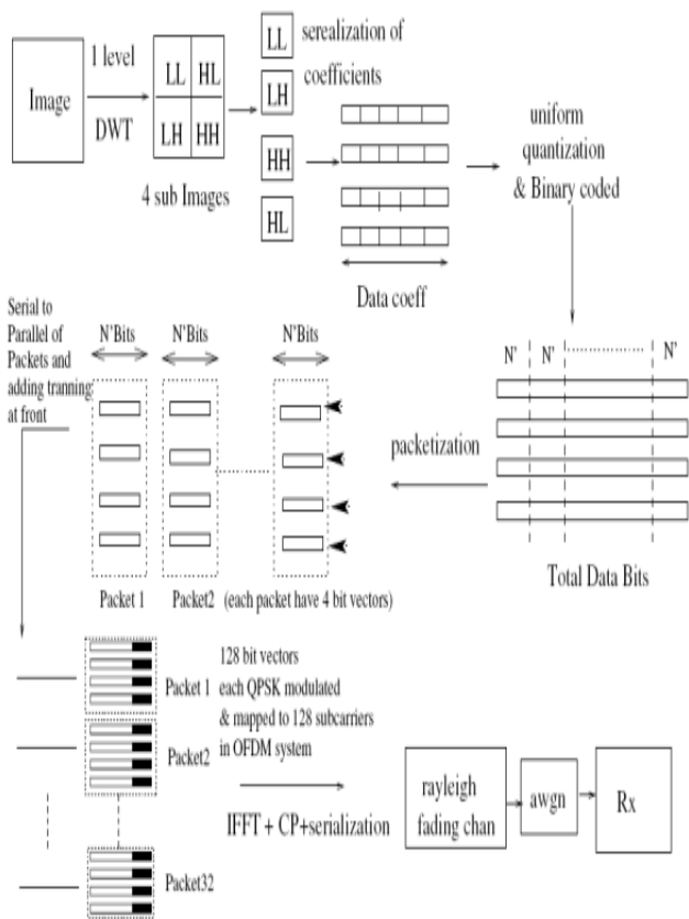
Fig. 2 DWT-OFDM SYSTEM
