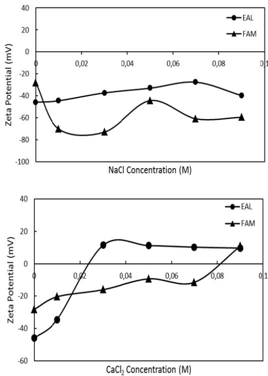
Fig. 2 Effects of electrolytes on zeta potential
