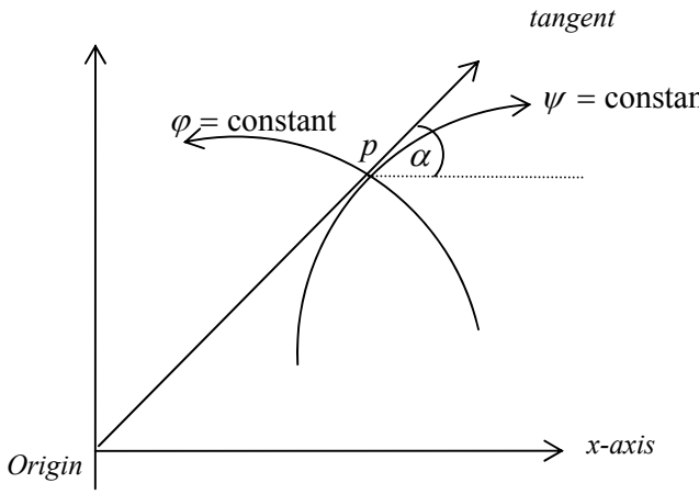
Fig. 1 ( \phi, \psi ) coordinate system
