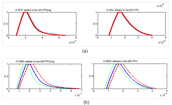
Fig. 9 The SIS PFD avg and PFH confidence intervals for (a) n = 1E+4 and (b) n = 20
