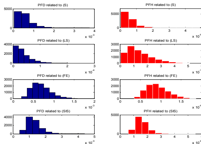
Fig. 1 Histograms related to PFD avg and PFH
