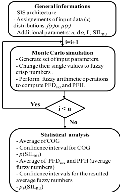
Fig. 5 Overall process for combining MC and fuzzy sets
