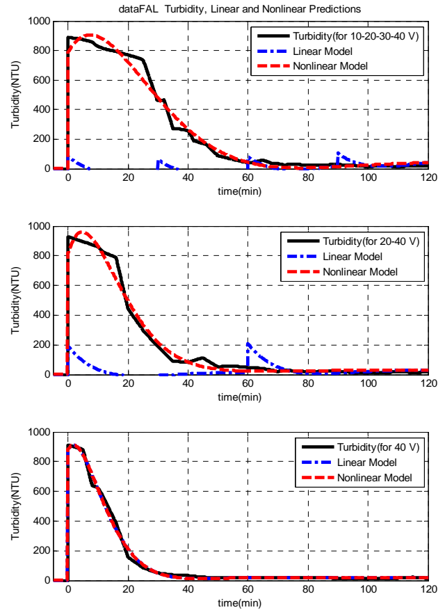
Fig. 7 The turbidity measurements and the linear and nonlinear model predictions (FAL wastewaters)
