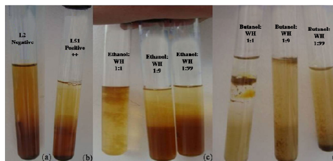
Fig. 4 Qualitative ethanol determination in medium with water hyacinth at 10% as measured by Iodoform test (a) Negative Iodoform test (b) Positive Iodoform test (++) (c) Ethanol Control (d) Butanol Control
