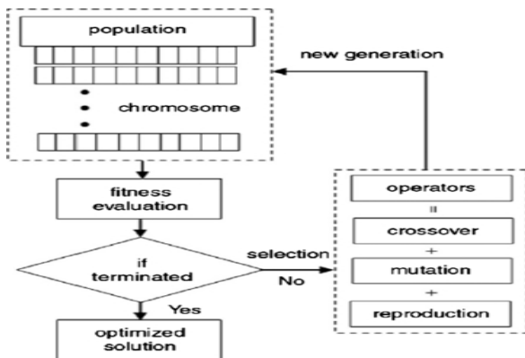
Fig. 1 Evolutionary Algorithm Flow Chart
