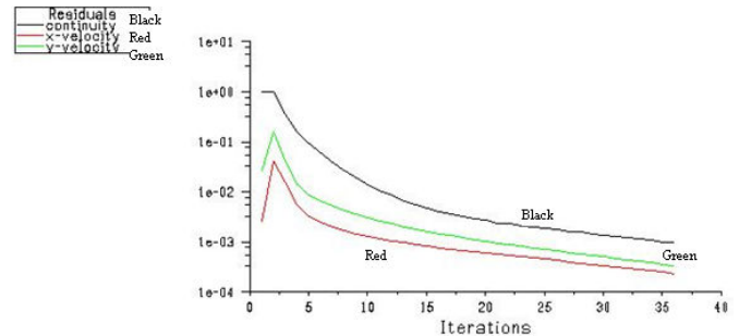
Fig. 6 Velocity iteration plot to check convergence
