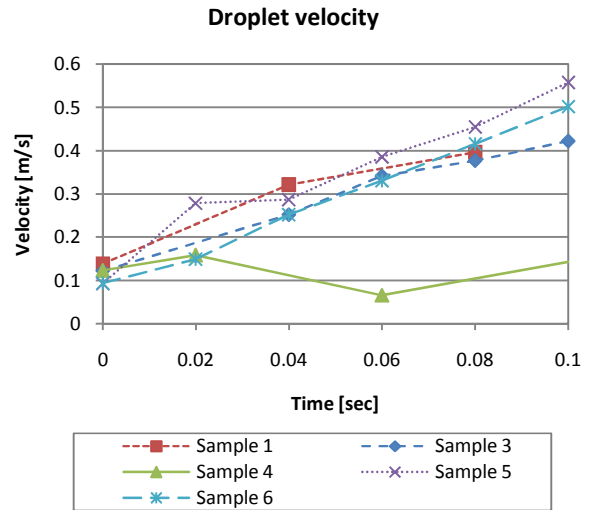
Fig. 2 The velocity of the droplet movement on inclined surface under 20°
