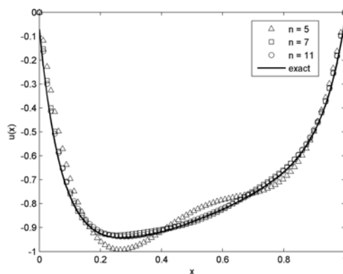
Fig. 13. Exact and numerical solutions, \varepsilon = 0.005 , analysis case C2
