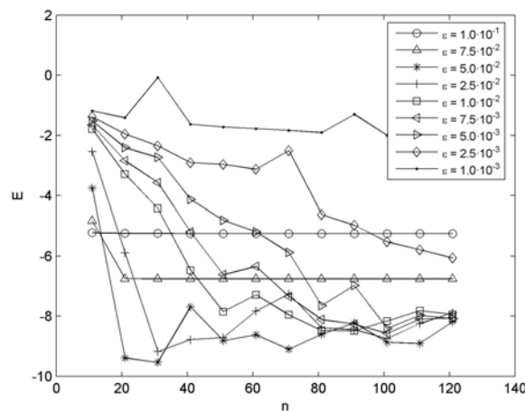
Fig. 8. Norm of error E , analysis case B
