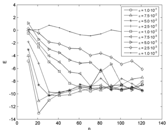
Fig. 5. Norm of error E , analysis case A
