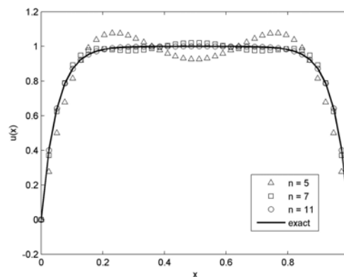
Fig. 6. Exact and numerical solutions, \varepsilon = 0.05 , analysis case B
