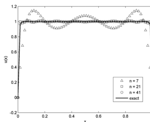
Fig. 7. Exact and numerical solutions, \varepsilon = 0.005 , analysis case B
