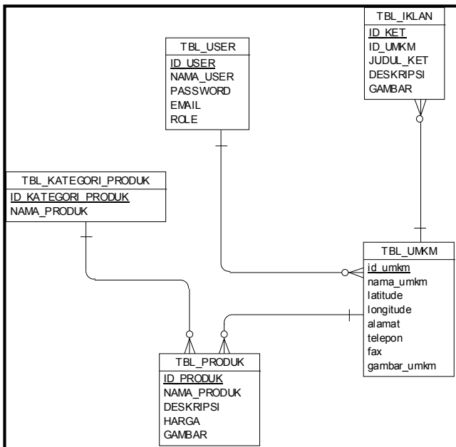
Fig. 6 Entity Relationship Diagram
